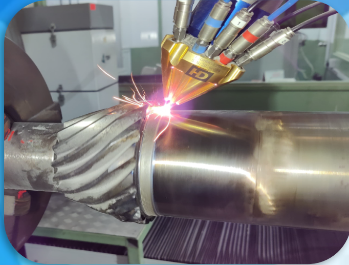
LASER CLADDING FOR 5 JOURNALS
